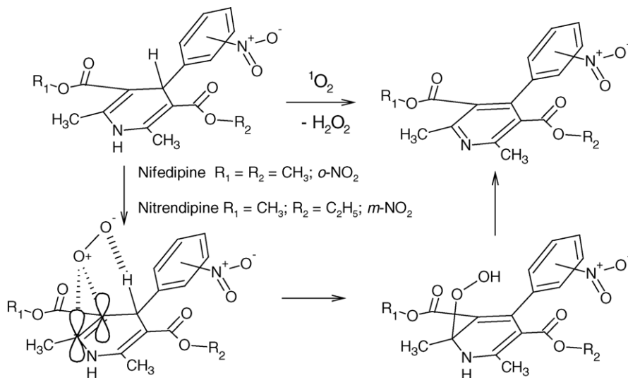
Fig. 9. Proposed mechanism for the reaction of O_2(^1\Delta_g) with nitrendipine and nifedipine.
